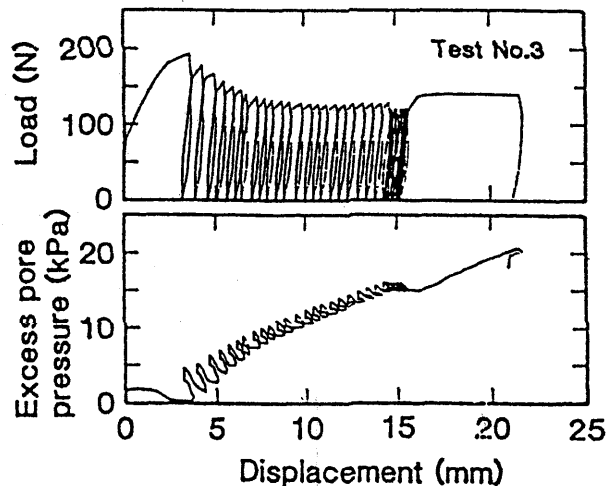
Fig.4 Test Results of Test No.3.
