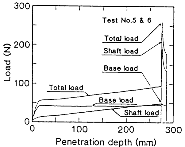
Fig.6 Load and Penetration Depth in Test Nos.5 & 6.
