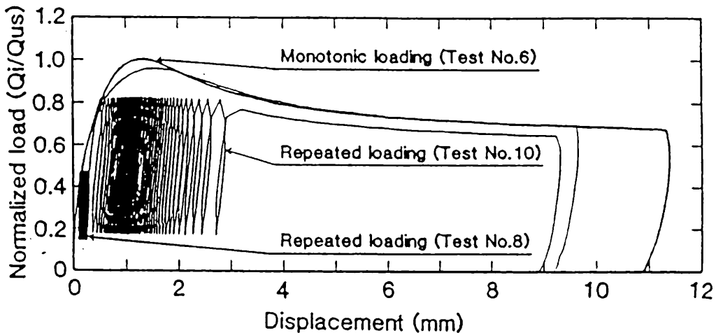
Fig.7 Load-Displacement Relationships in Test Nos.6,8,10.
