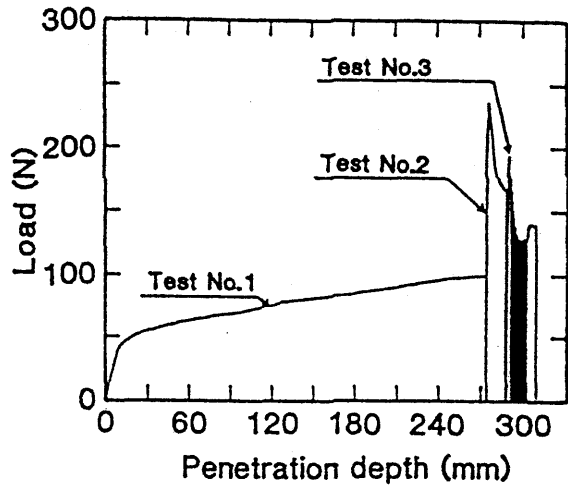
Fig.2 Load and Penetration Depth in Test Nos.1,2,3.
