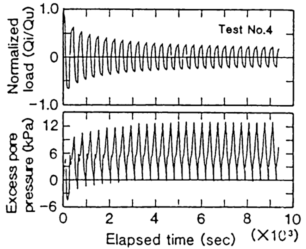
Fig.5 Test Results of Test No.4.
