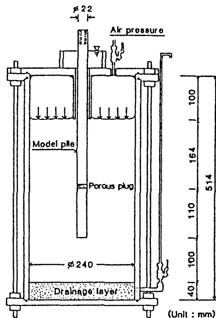
Fig.1 Testing Apparatus and Pile-I.
