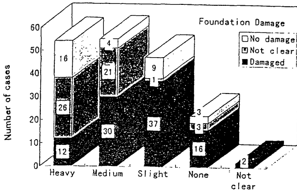
Figure 1 Relation to Superstructure Damage
