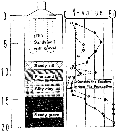
(a) Ground Condition and Pile Layout
