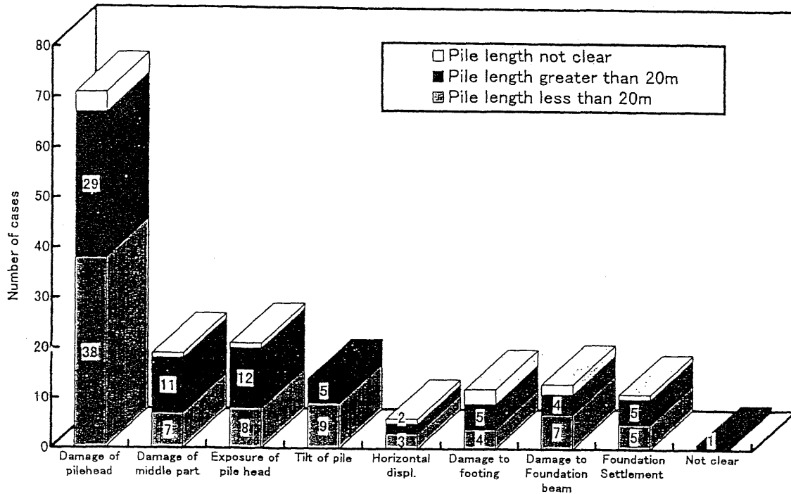
Figure 5 The nature of Pile Foundation Damage and the Pile length
