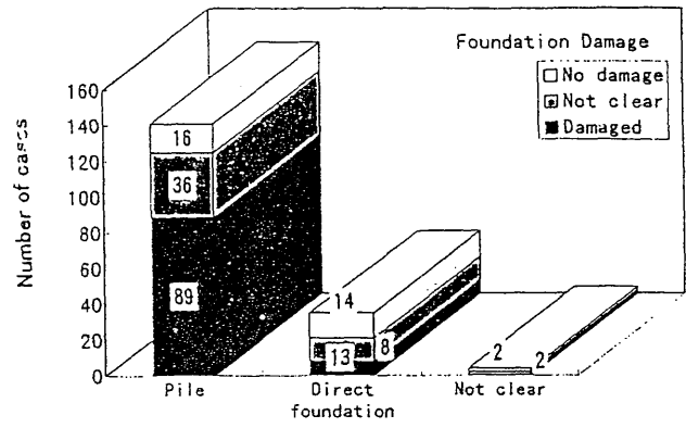
Figure 2 Pile & Direct Foundations
