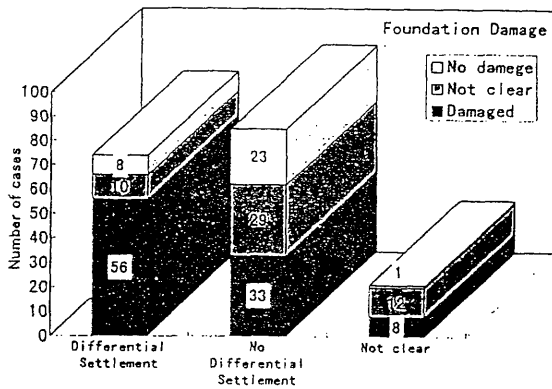
Figure 3 Relation to the Differential Settlement in the Vicinity
