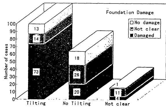
Figure 4 Relation to Tilting in the Building Superstructure
