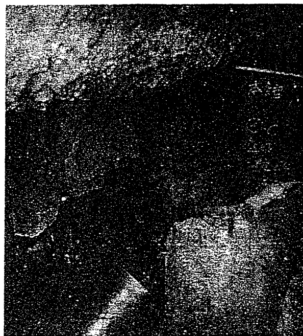
(b) \phi 350 PC Pile in Ordinary Ground with Large Settlement due to Lateral Spreading
